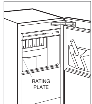
Ice machine.
